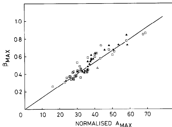
Fig.1. The correlation of the slow phase ( \beta_{max} ) with the normalised A_{max} . The data were obtained by either cation-induced (□) or LHCP phosphorylation-induced (▲) fluorescence changes. The line is the least squares fit to the experimental points with a correlation coefficient ( r ) of 0.94.
